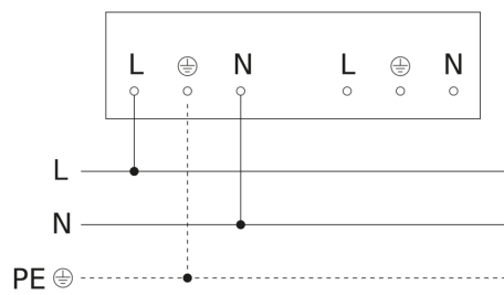
Circuit diagram 1
